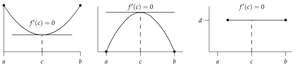
Figure 30.4: When the hypotheses of Rolle's theorem are satisfied, there is a horizontal tangent, i.e., a critical point exists.
