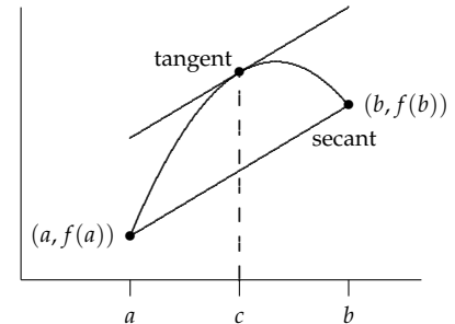
Figure 30.5: Under the conditions of the MVT, there's a point c in (a, b) so that the secant slope f'(c) = \frac{f(b) - f(a)}{b - a} equals the tangent slope f'(c) .
