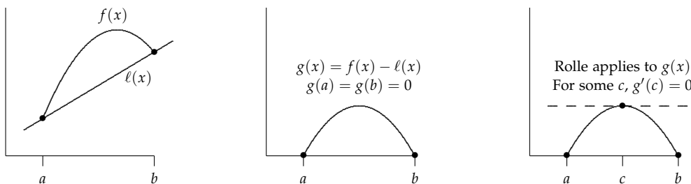
Figure 30.6: f(x) and \ell(x) have the same value at the endpoints a and b so their difference is 0 at both a and b . Consequently Rolle's theorem applies to g and there is a point c between a and b such that g'(c) = 0 .
